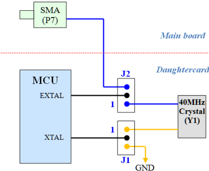
Figure 8. EVB Clock Selection
