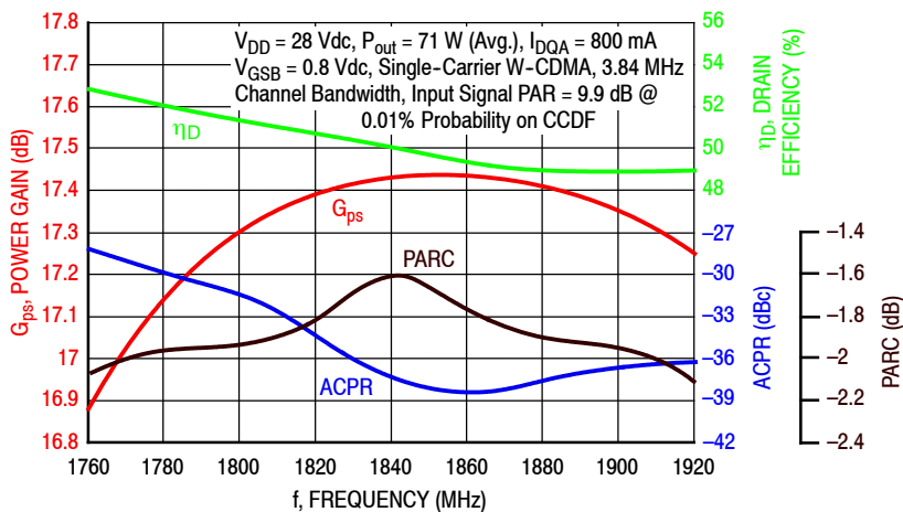
Figure 3. Single-Carrier Output Peak-to-Average Ratio Compression (PARC) Broadband Performance @ P_{out} = 71 \text{ Watts Avg.}
