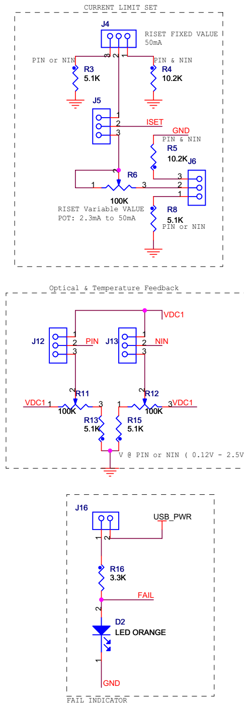
Figure 10. EVb Schematic (3)
