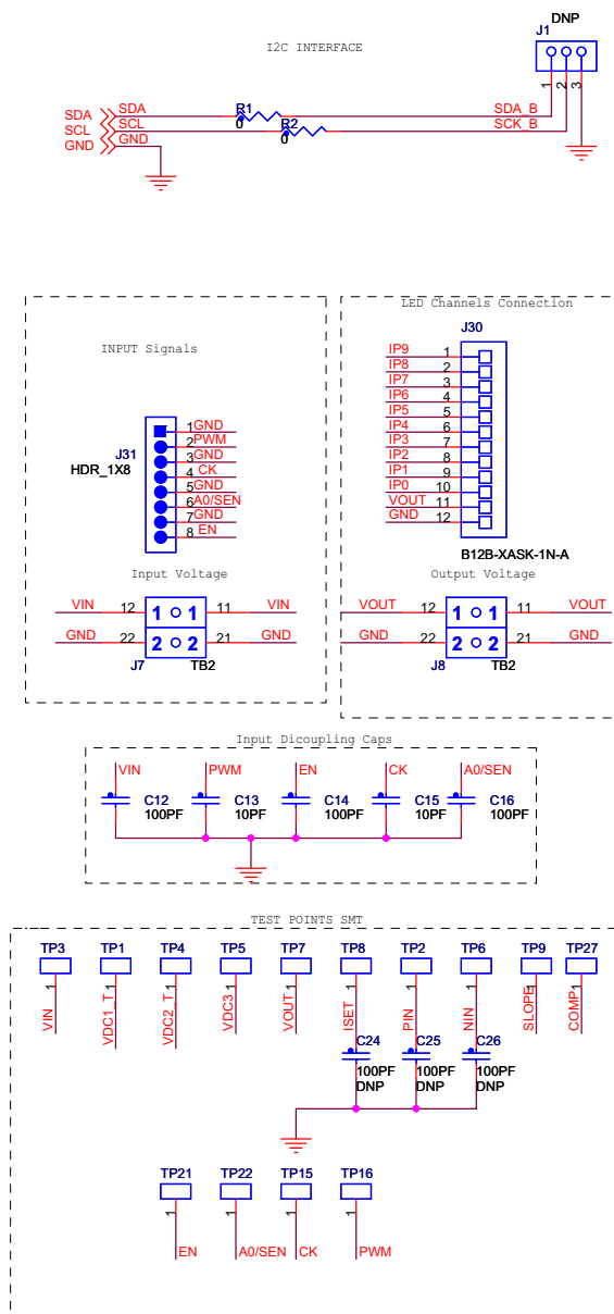
Figure 9. EVB Schematic (2)
