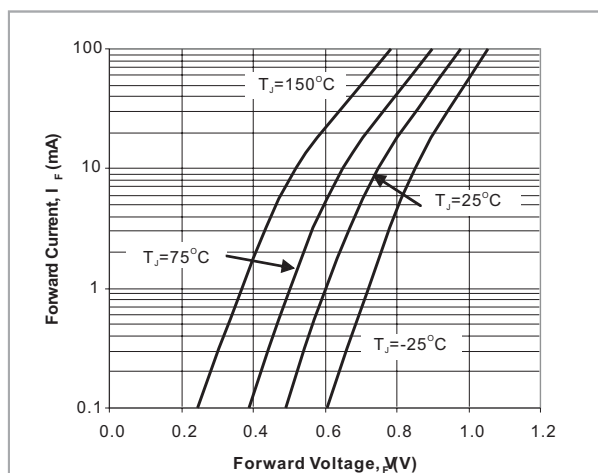
Fig. 3. Forward Current vs. Forward
