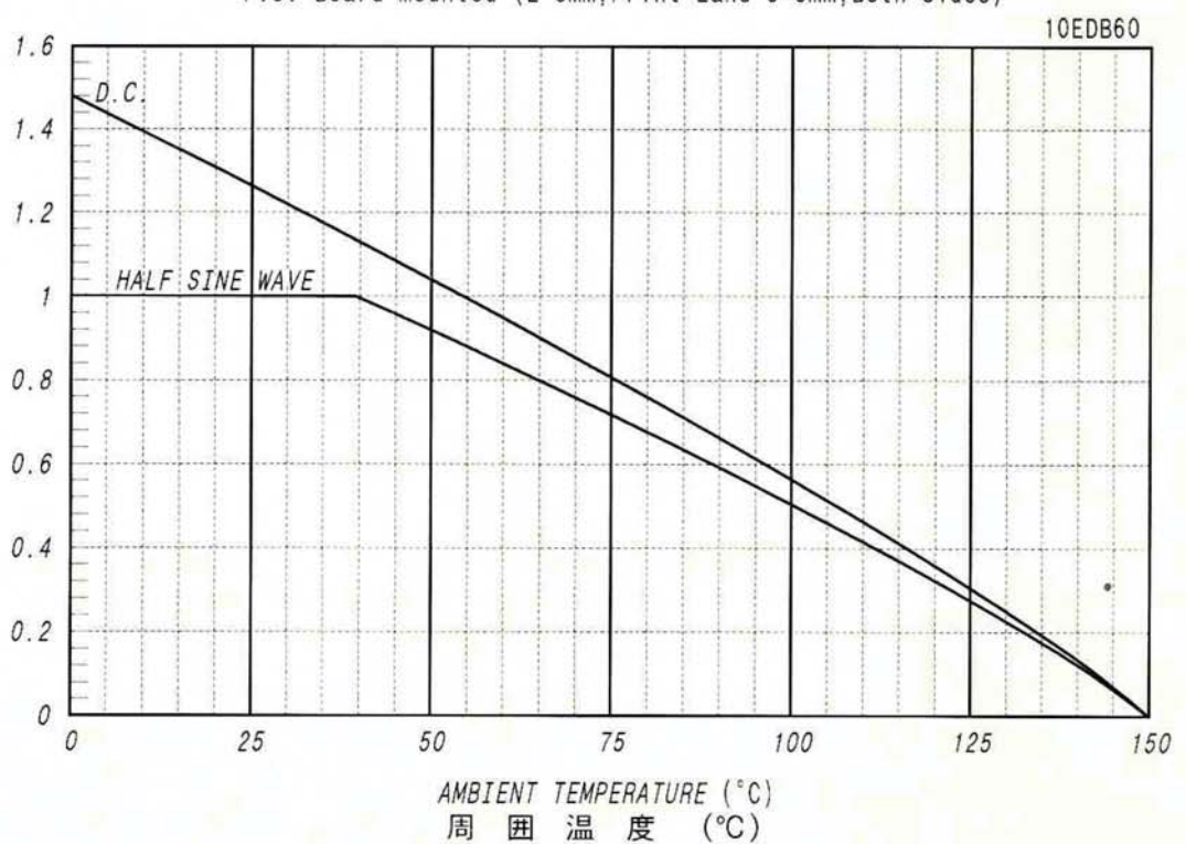
平均順電流一周圍溫度定格 AVERAGE FORWARD CURRENT VS. AMBIENT TEMPERATURE
