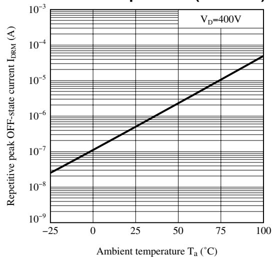
Fig.7-a Repetitive Peak OFF-state Current vs. Ambient Temperature (S102T01)
