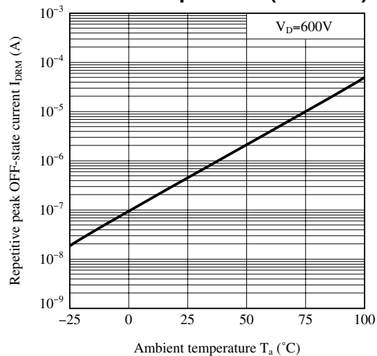
Fig.7-b Repetitive Peak OFF-state Current vs. Ambient Temperature (S202T01)
