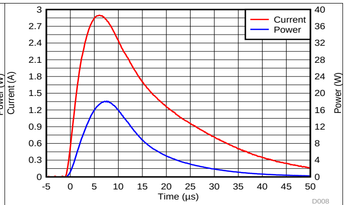
Figure 8. Surge Curves, GND to IO
