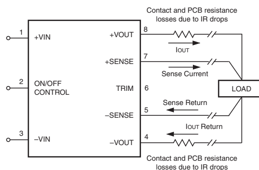
Figure 4. Remote Sense Circuit Configuration
