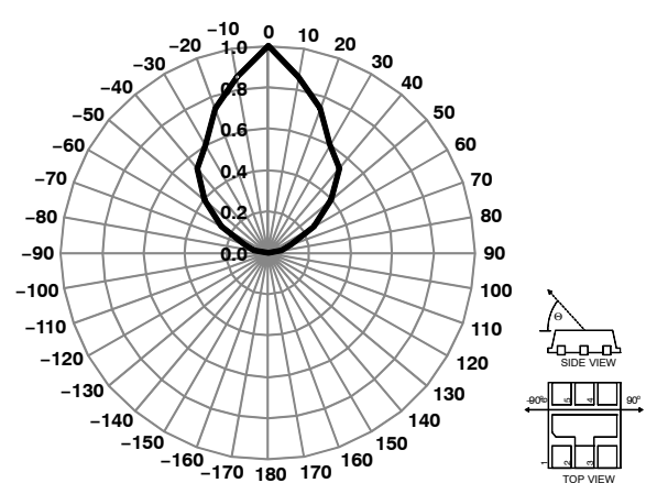
Figure 9. Output Counts vs. Angle (Side View, Normalized)
