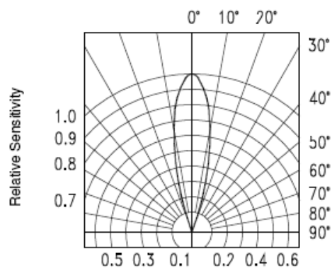
FIG.5 SENSITIVITY DIAGRAM
