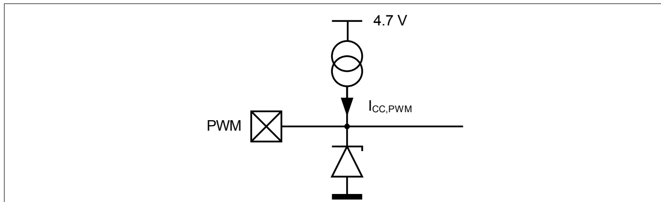
Figure 4 PWM Input
