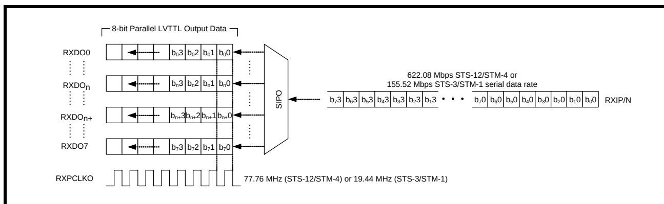
FIGURE 8. SIMPLIFIED BLOCK DIAGRAM OF SIPO
