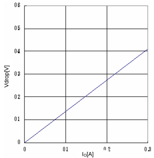
Fig.22 Minimum dropout Voltage 2 ( V_{CC}=4.5\text{V} , T_a=25^\circ\text{C} )
