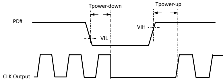
Figure 13. Output Enable/ Disable and Power Down Functions
