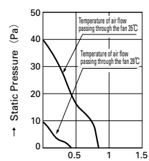
→ Air Flow (m 3 /min) 109P0812T6H122(123)
