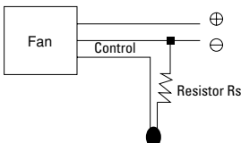
Fig. 3 Recommended thermistor
