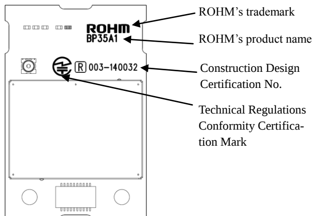
Fig. 8. Marking Specification
