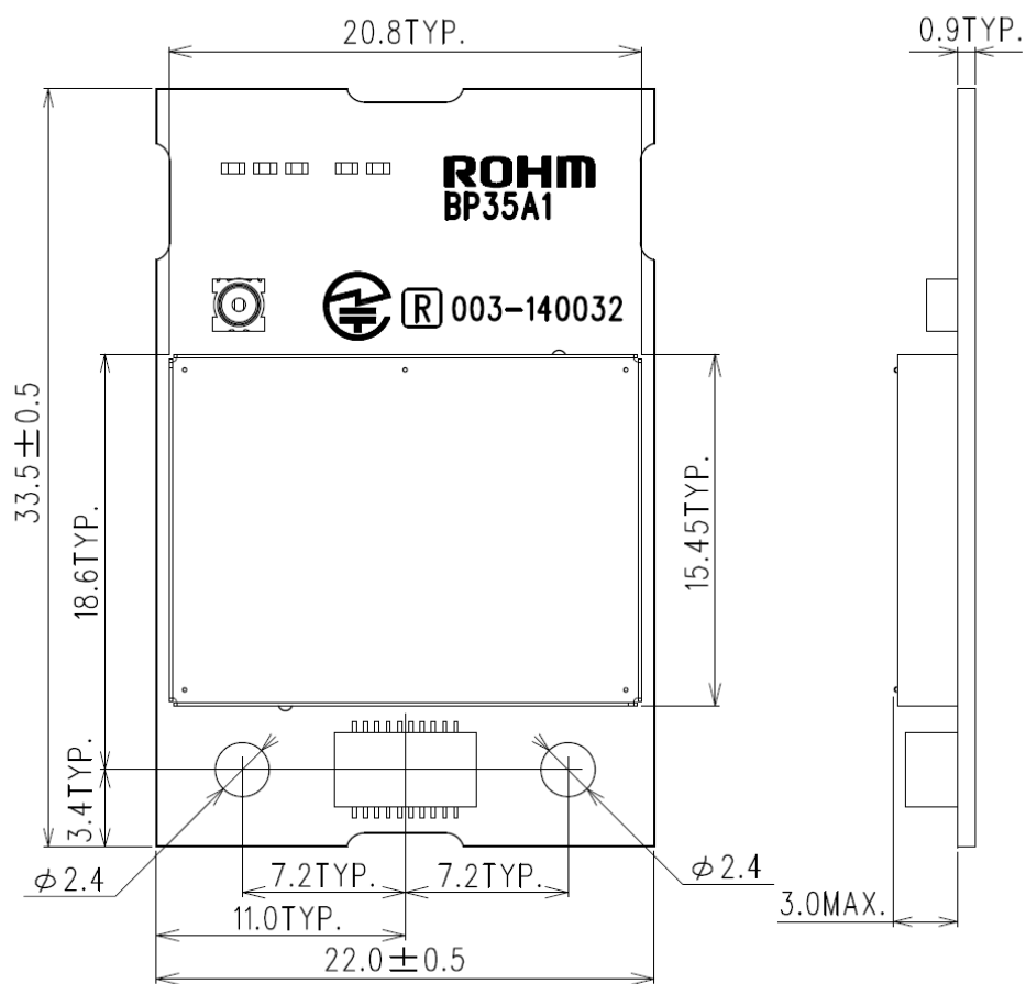
Fig. 7. Outline Dimensions Diagram
