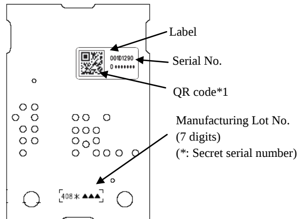
Fig. 8. Marking Specification
