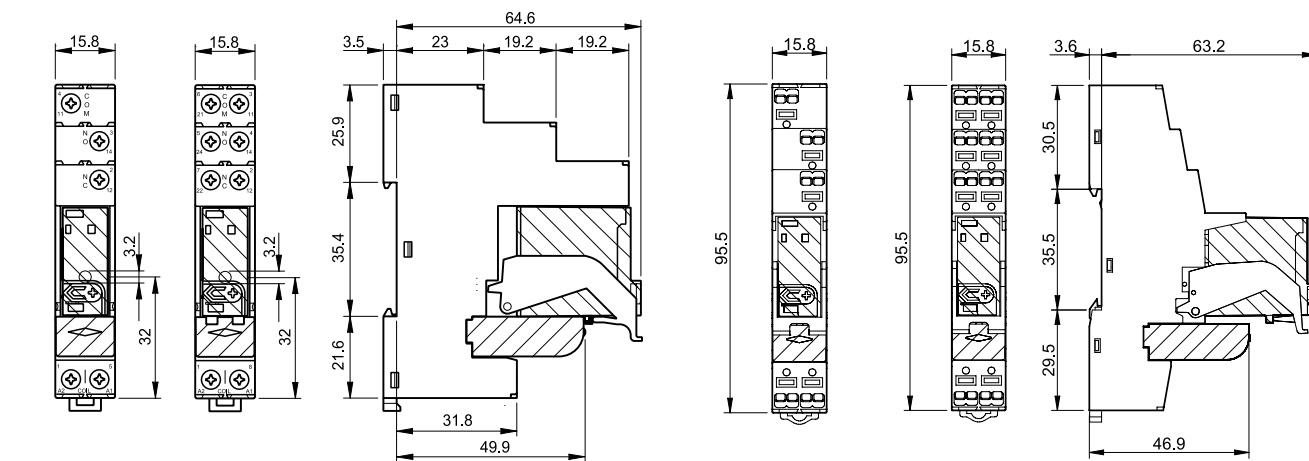
Types 4C.01/4C.02 Box clamp
