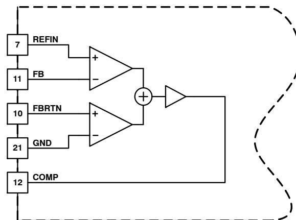
Figure 4. Differential Error Amplifier
