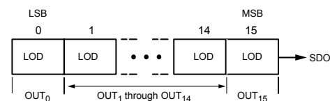
Figure 11. Individual output LOD data format
