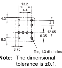
PCB Processing Dimensions (Bottom View)
