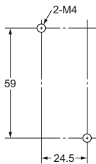
Mounting Hole Dimensions
