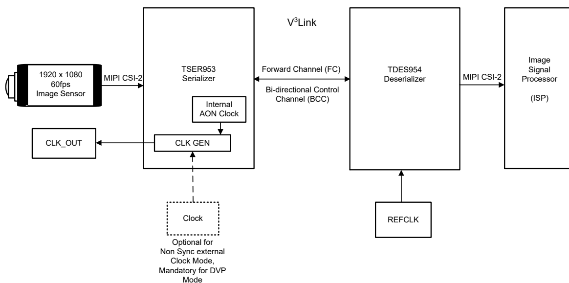
Figure 7-6. Clocking System Diagram
