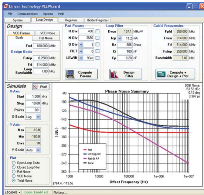
Figure 3. PLLWizard Screenshot
