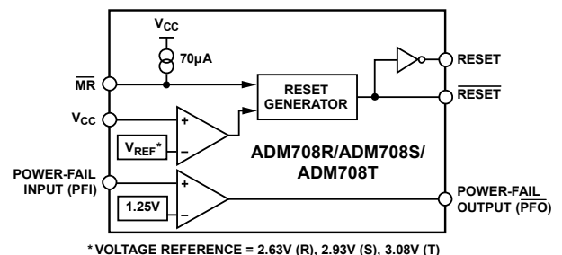
Figure 2. ADM708R/ADM708S/ADM708T
