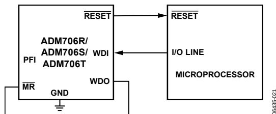
Figure 21. \overline{\text{RESET}} from WDO
