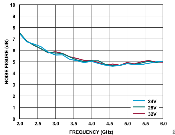
Figure 44. Noise Figure vs. Frequency for Various V_{DD} Values, I_{DQ} = 750\text{ mA}
