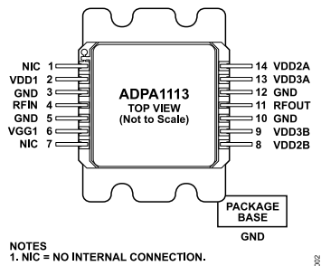
Figure 2. Pin Configuration
