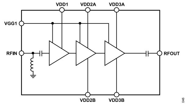
Figure 45. Basic Block Diagram
