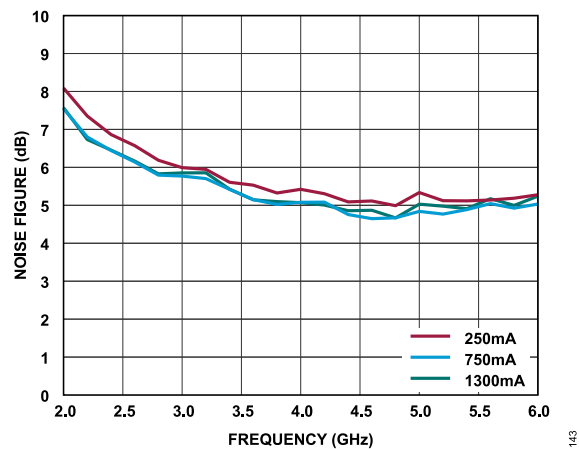
Figure 43. Noise Figure vs. Frequency for Various I_{DQ} Values, V_{DD} = 28\text{ V}
