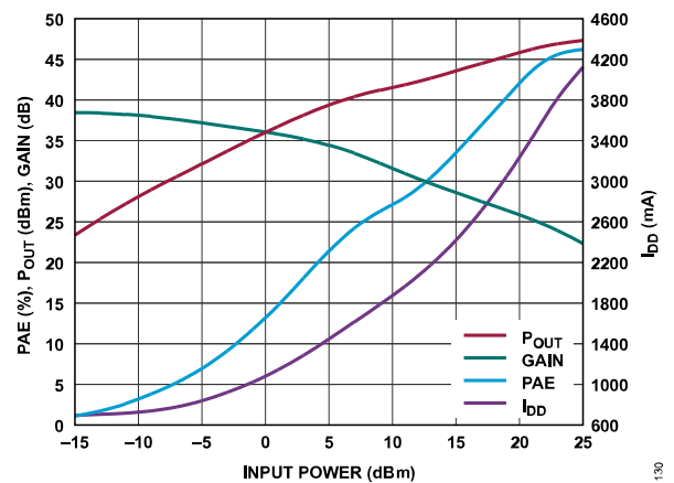
Figure 30. PAE, P_{OUT} , Gain, and Supply Current ( I_{DD} ) vs. Input Power at 2.0 GHz, V_{DD} = 28 V, I_{DQ} = 750 mA
