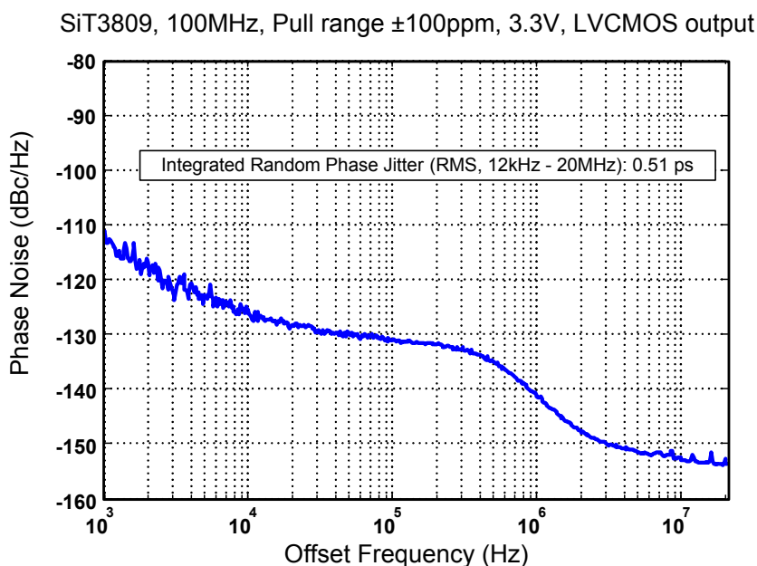
Figure 3. Phase Noise
