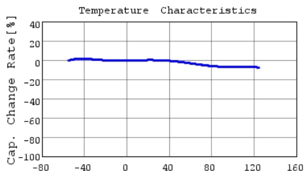
GCJ188R72A332KA01 C-Temp. capchange, DC0.0V,
