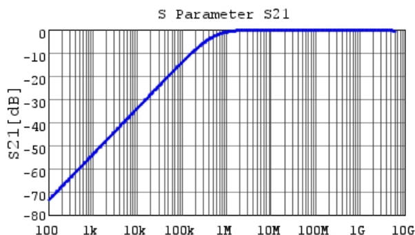
GCJ188R72A332KA01 S21 DC0V,25degC
