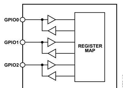
Figure 116. GPIOx Pin Functionality
