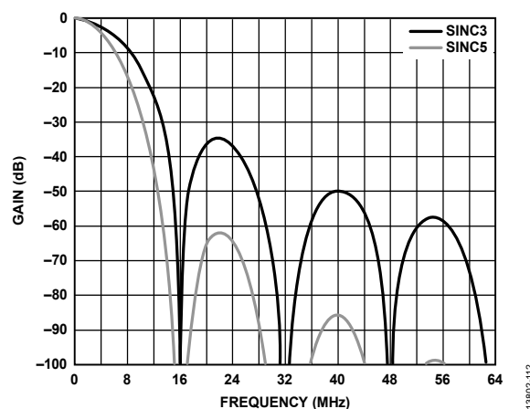
Figure 112. Sinc3/Sinc5 Frequency Response in Low Power Mode
