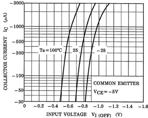
Fig. 10.4 RN2307 I_C - V_{I(OFF)}
