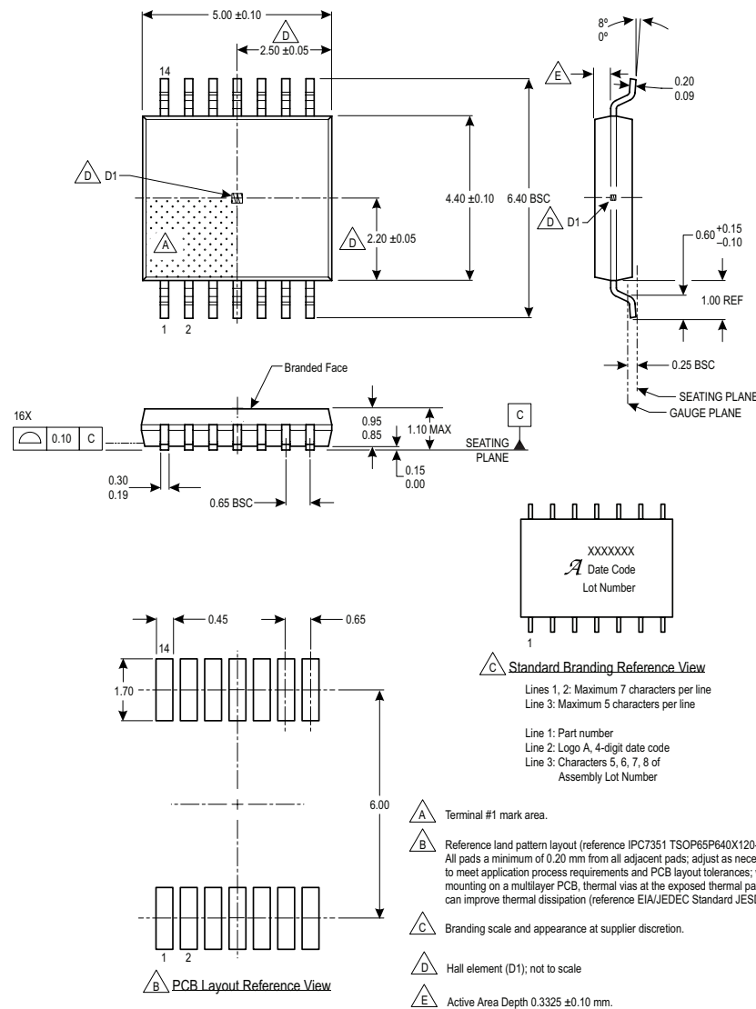
Figure 33: Package LE, 14-Pin TSSOP, single die
