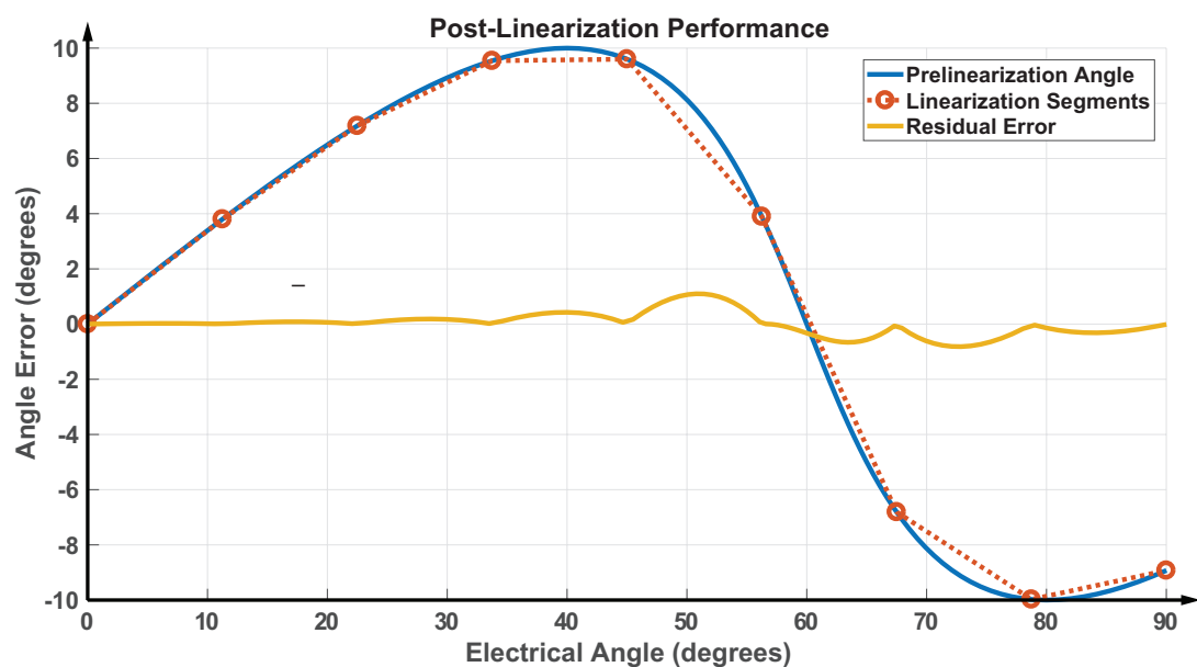
Figure 8: Post-Linearization Error
