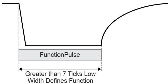
Figure 46: Function Pulse (Output by Host)
