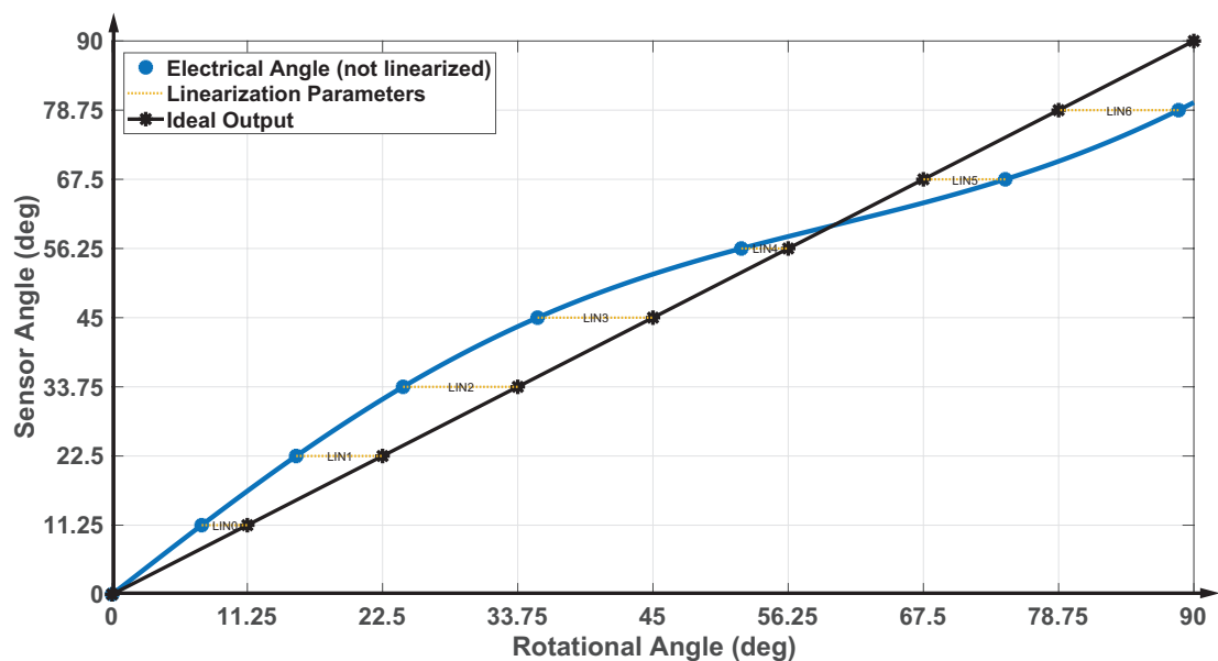
Figure 7: Linearization Example
