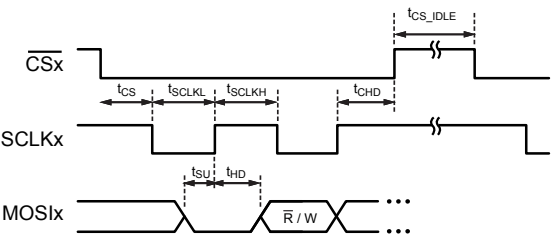
Figure 15: A33002 SPI Interface Timings Input
