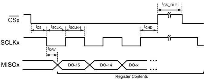
Figure 16: A33002 SPI Interface Timings Output
