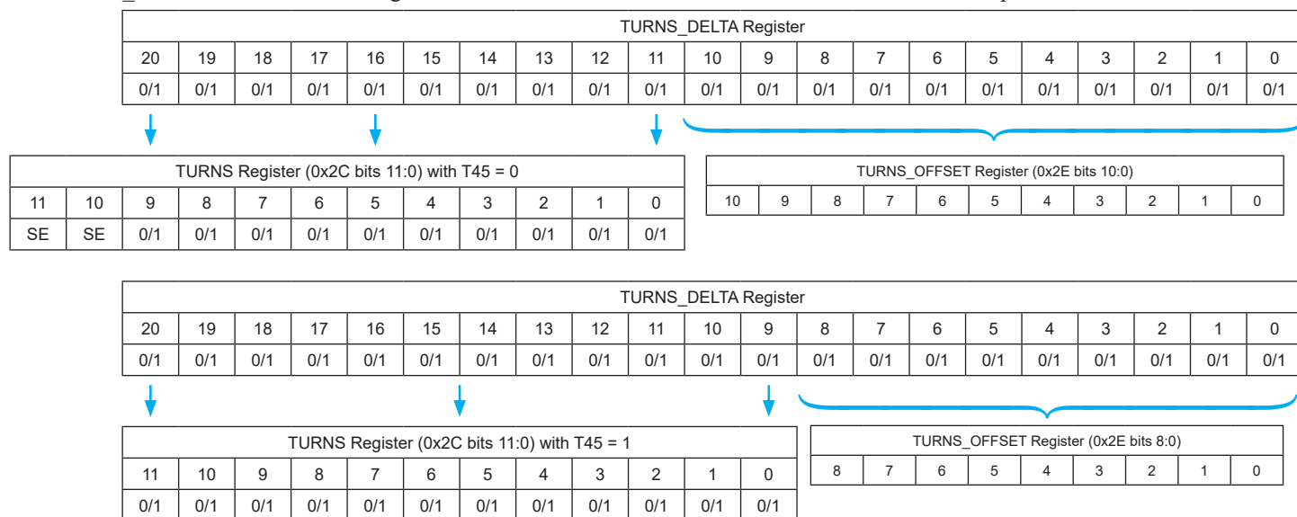
Figure 12: Turns Register
