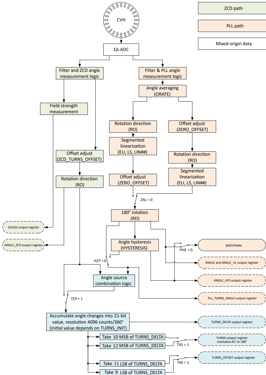
Figure 6: Angle Measurement – Sensor Readout Steps
