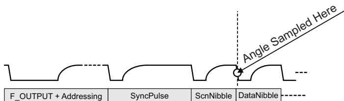
Figure 52: Sample-on-Output Example
