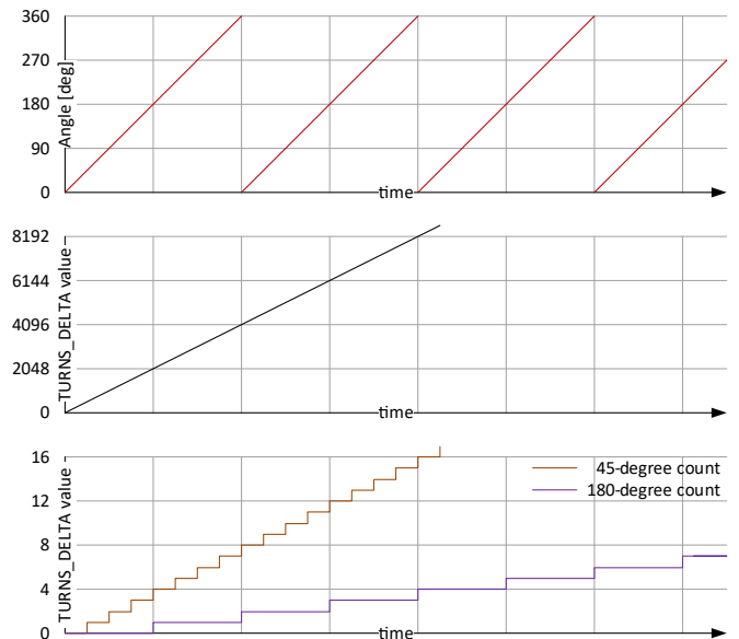
Figure 10: Turns Counting
