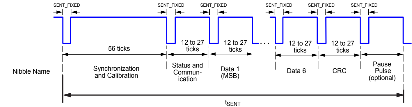
Figure 37: General Format for SENT Message Frame
