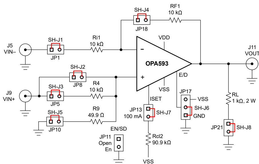
Figure 4-2. Simplified Schematic of OPA593EVM Amplifier Default Configuration
