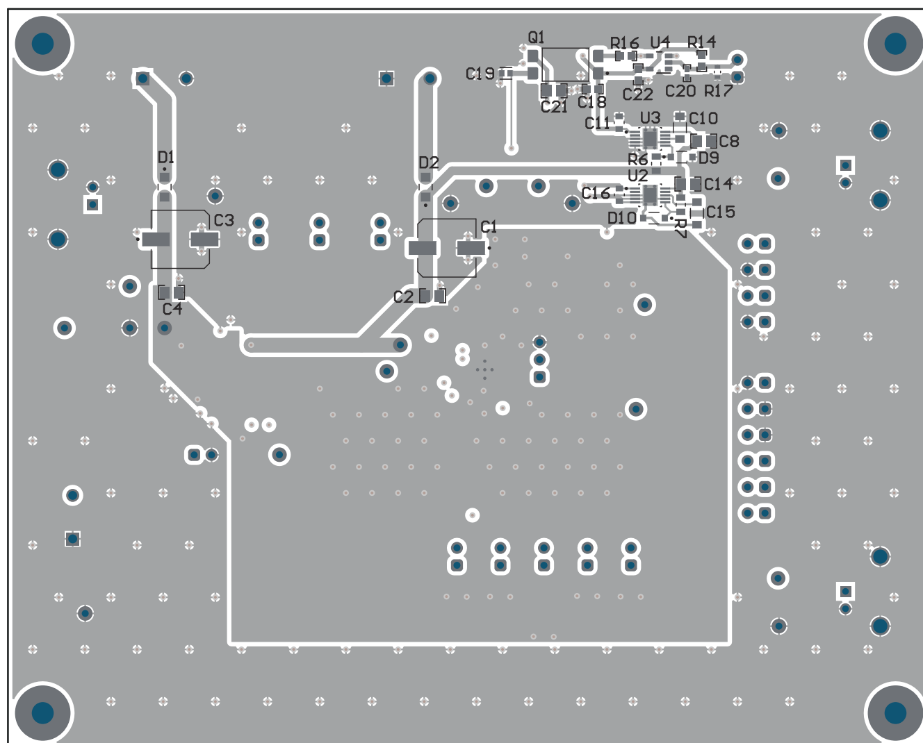
Figure 4-4. Bottom-Side View of the OPA593EVM PCB
