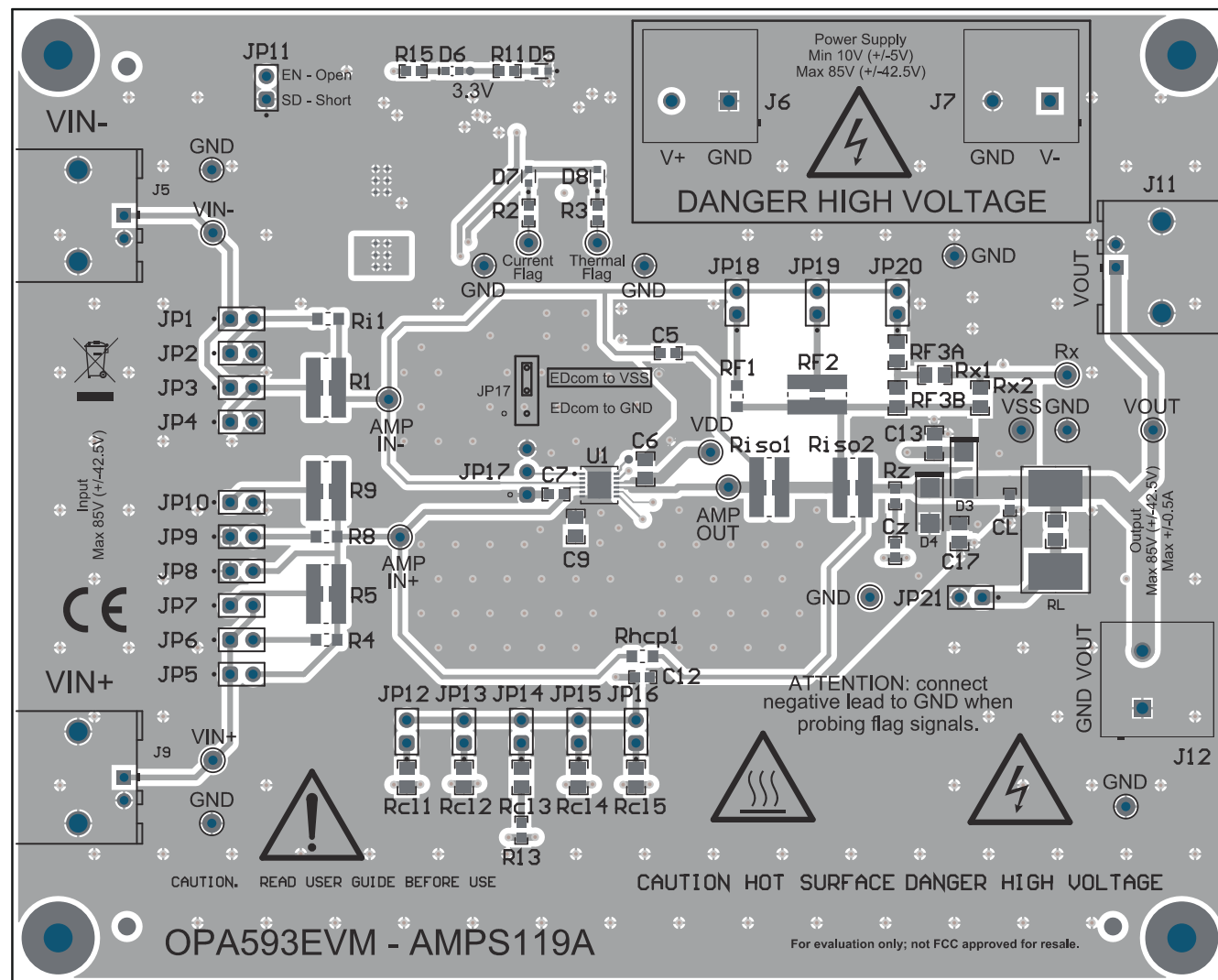
Figure 4-3. Top-Side View of the OPA593EVM PCB
