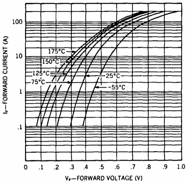
Typical Forward Current vs Forward Voltage
