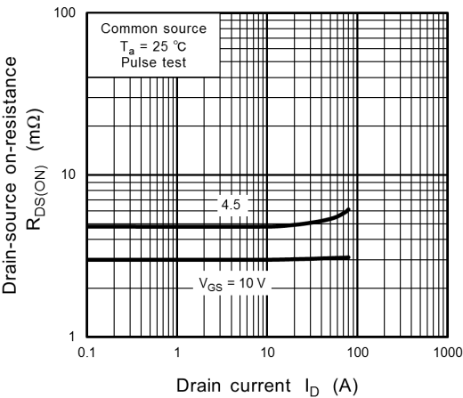
Fig. 8.8 R_{DS(ON)} - I_D
