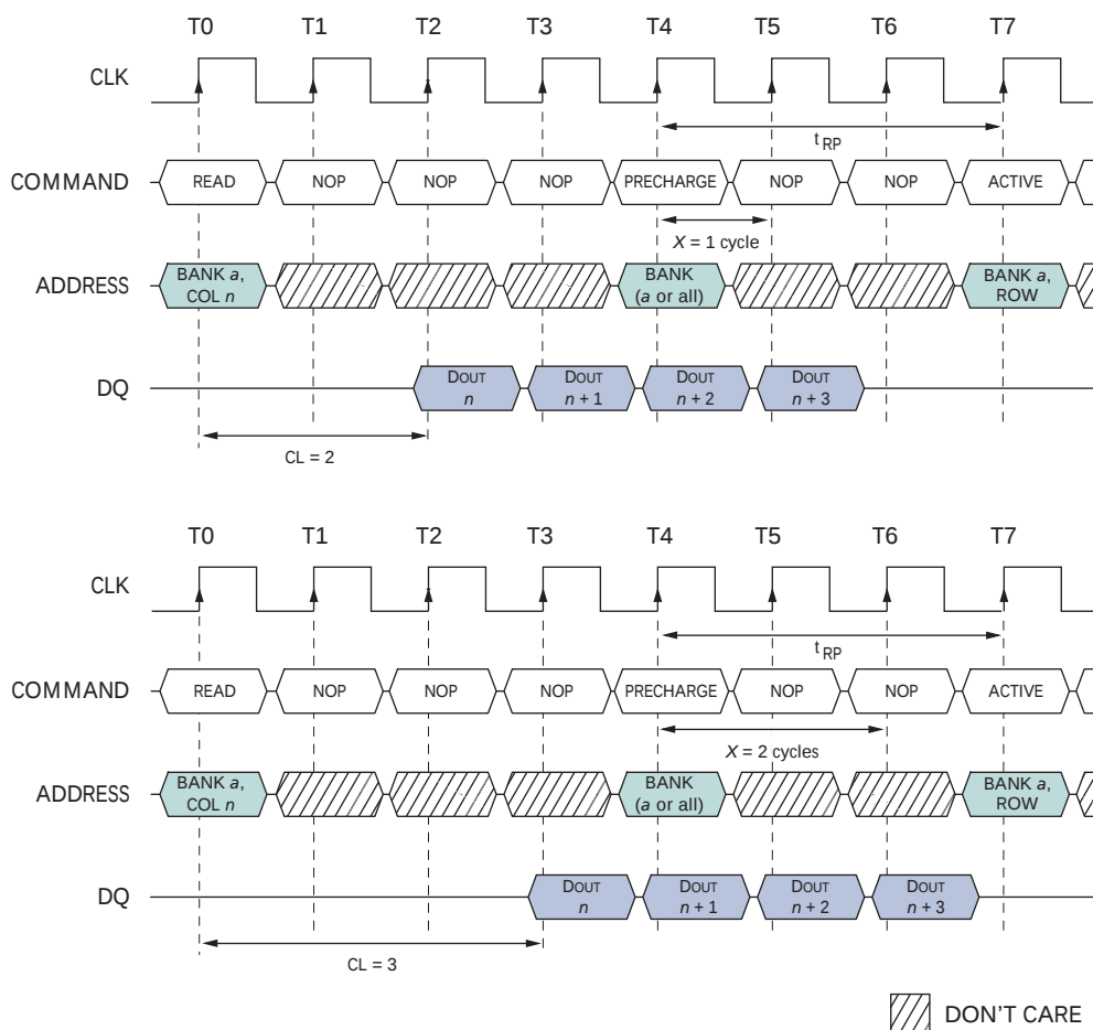
Figure 16: READ-to-PRECHARGE
