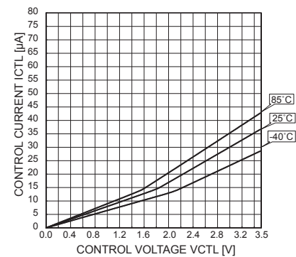
Fig.10 Control sink current
