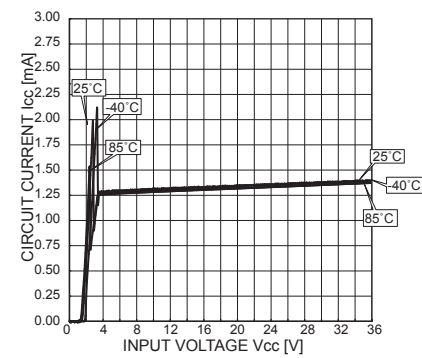
Fig.5 Circuit current
