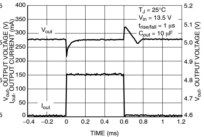
Figure 15. Load Transient
