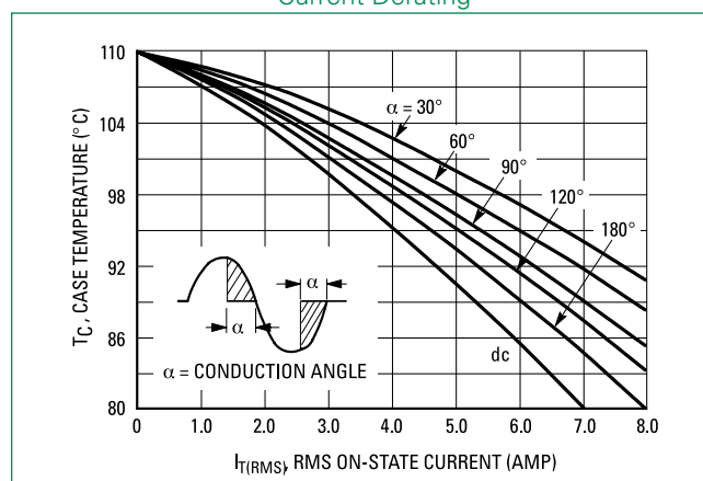
Figure 1. Current Derating
