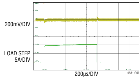
Single Channel Load Transient Response (10A) to (20A) Load Step, 10\text{A}/\mu\text{s} 12\text{V} , V_{\text{OUT}} = 3.3\text{V} , f_{\text{SW}} = 500\text{kHz}
