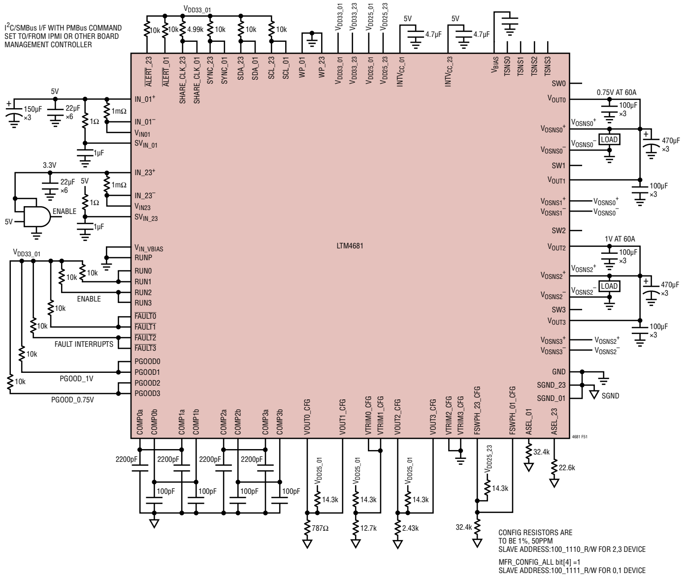
Figure 51. 1V/60A and 0.75V/60A Outputs Generated from 3.3V and 5V Power Input and Providing I^2C /SMBus/PMBus Serial Interface
