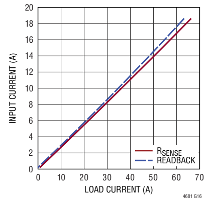
Supply Current vs Load Current Comparison, R_{\text{SENSE}} = 2\text{m}\Omega , 12\text{V} to 3.3\text{V}_{\text{OUT}} , 650\text{kHz}
