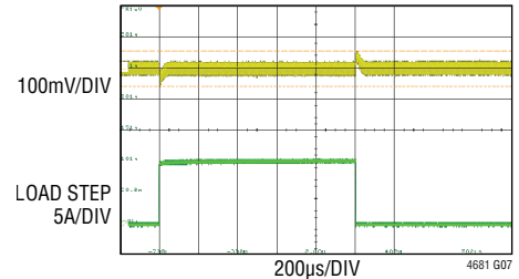
Single Channel Load Transient Response (10A) to (20A) Load Step, 10\text{A}/\mu\text{s} 12\text{V} , V_{\text{OUT}} = 1.5\text{V} , f_{\text{SW}} = 350\text{kHz}
