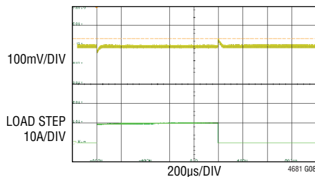
Single Channel Load Transient Response (10A) to (20A) Load Step, 10\text{A}/\mu\text{s} 12\text{V} , V_{\text{OUT}} = 2.5\text{V} , f_{\text{SW}} = 500\text{kHz}
