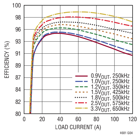
Quad Channel Single Output Efficiency V IN = S V IN = 12V, RUNP = 0V, V BIAS = 5.5V External, CCM Mode
