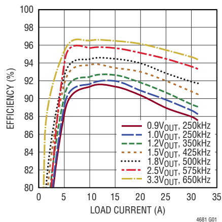
Single Channel Efficiency, 5V IN , V IN = S V IN = INT V CC = 5V, RUNP = 0V, CCM Mode
