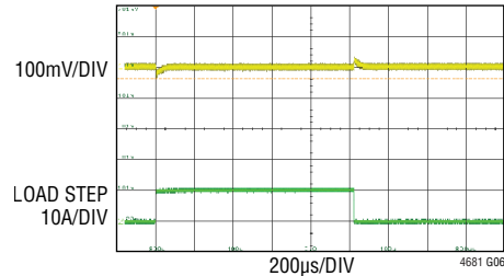
Single Channel Load Transient Response (10A) to (20A) Load Step, 10\text{A}/\mu\text{s} 12\text{V} , V_{\text{OUT}} = 1.2\text{V} , f_{\text{SW}} = 350\text{kHz}
