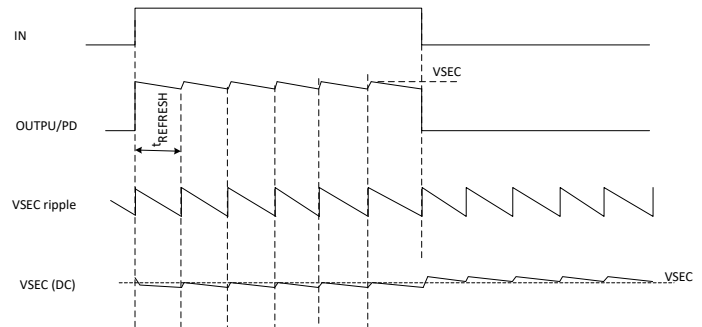
Figure 6: Refresh Mechanism
