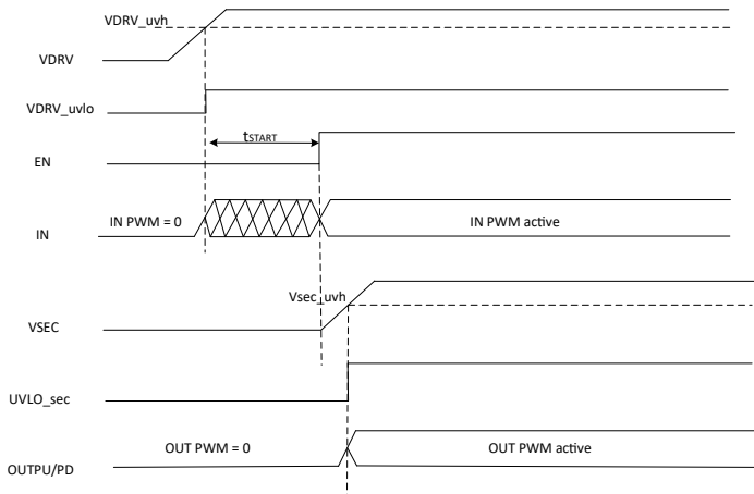
Figure 4: Startup Mechanism
