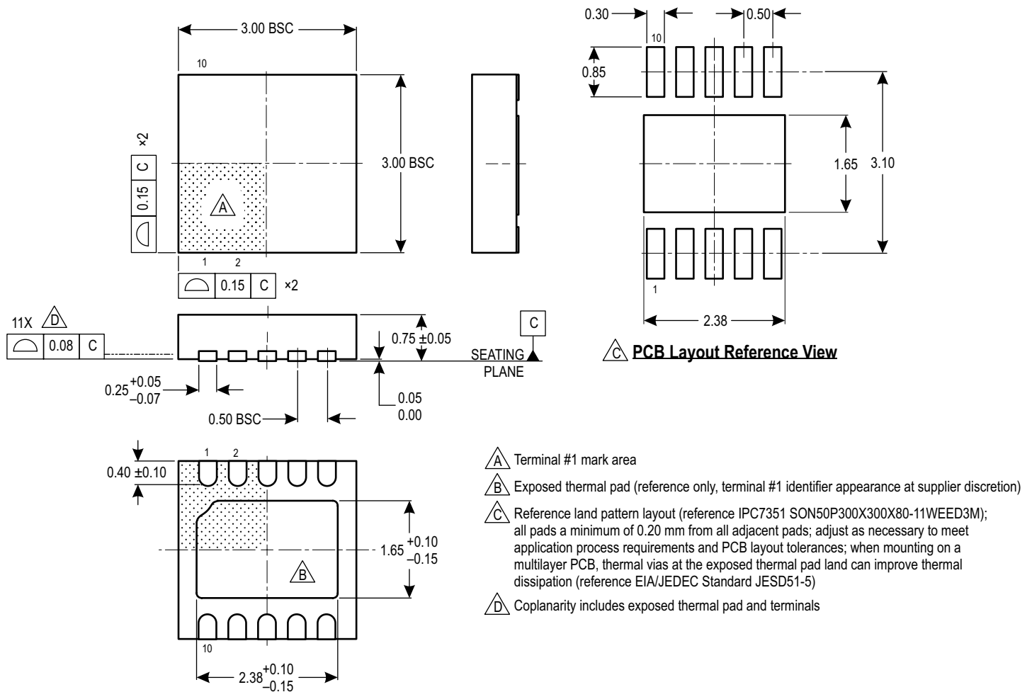
Figure 16: AHV85000 + AHV85040 EJ Package Outline and Recommended Footprint [4]
