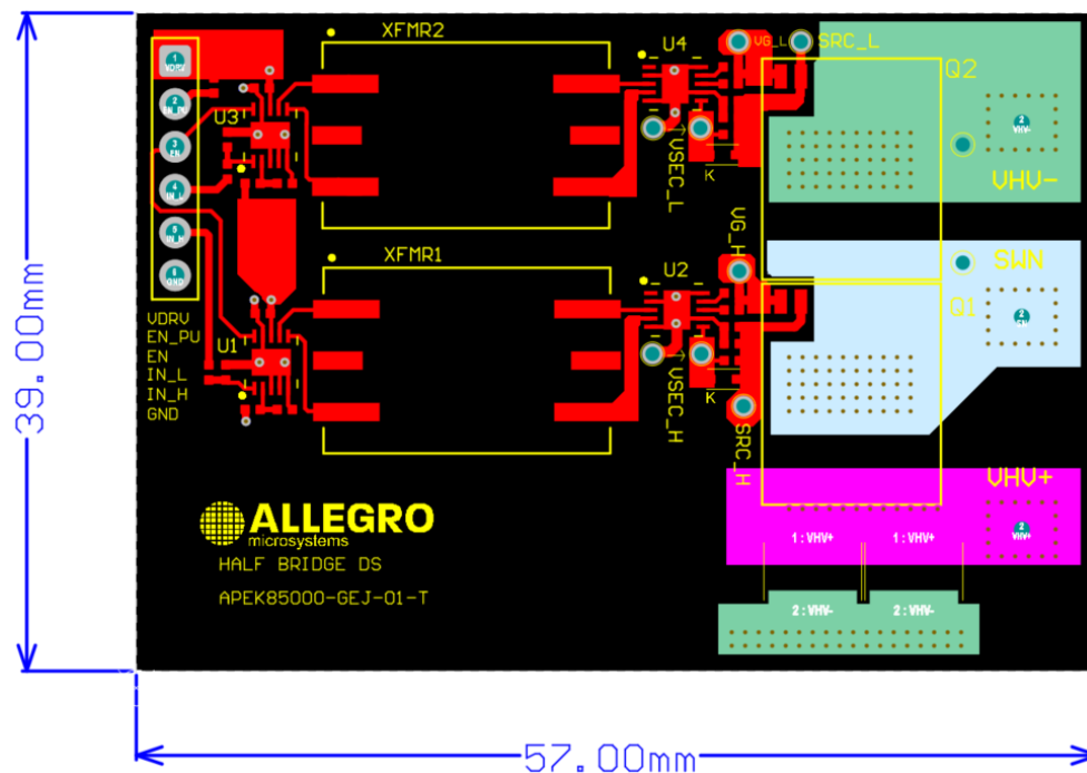
Figure 15: Example APEK85000-GEJ-01-T PCB Layout
