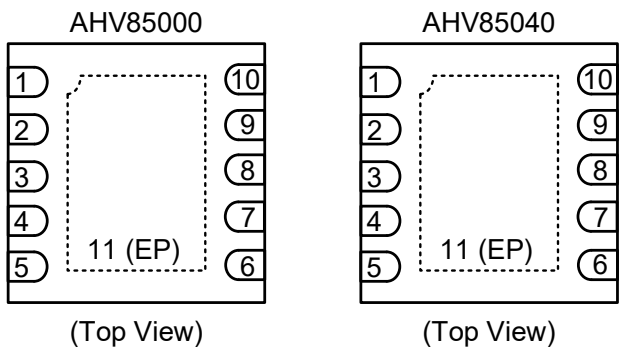
Package EJ Pinout (Top View)
