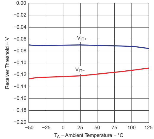
Figure 7-12. Receiver Threshold vs Ambient Temperature
