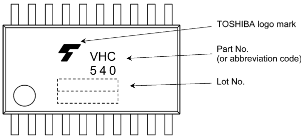
74VHC540FT
