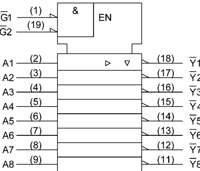
74VHC540FT
