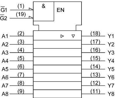
74VHC541FT
