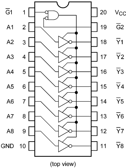
74VHC540FT
