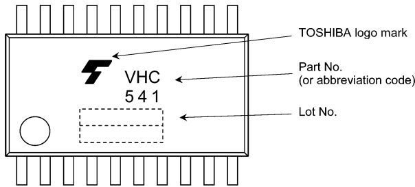
74VHC541FT
