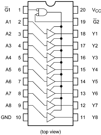
74VHC541FT
