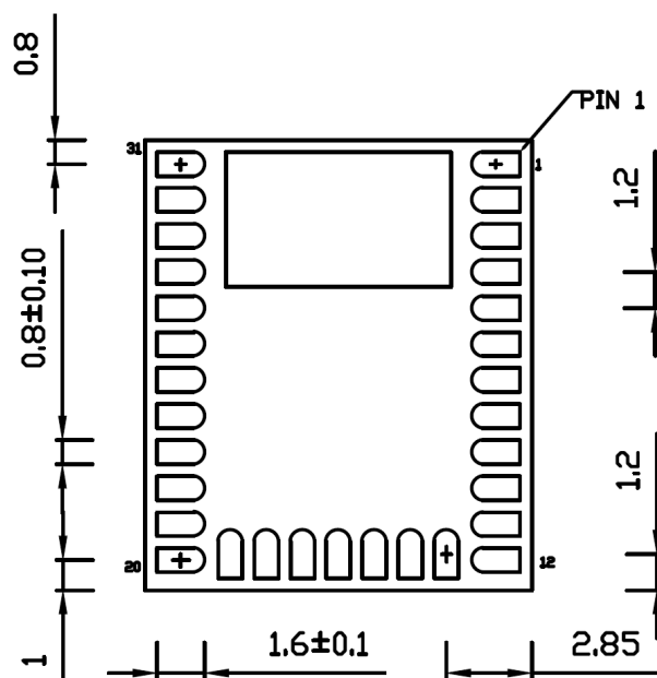
Figure 8.2. Bottom View
