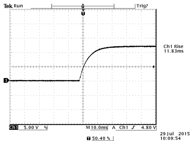
Figure 19. Rise time @ V_{in} = 24\text{ V} , Full Load
