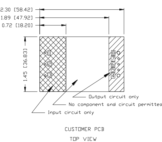
Figure 40. Recommended pad layout-1
