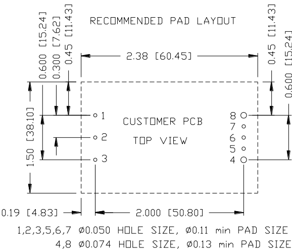
Figure 41. Recommended pad layout-2
