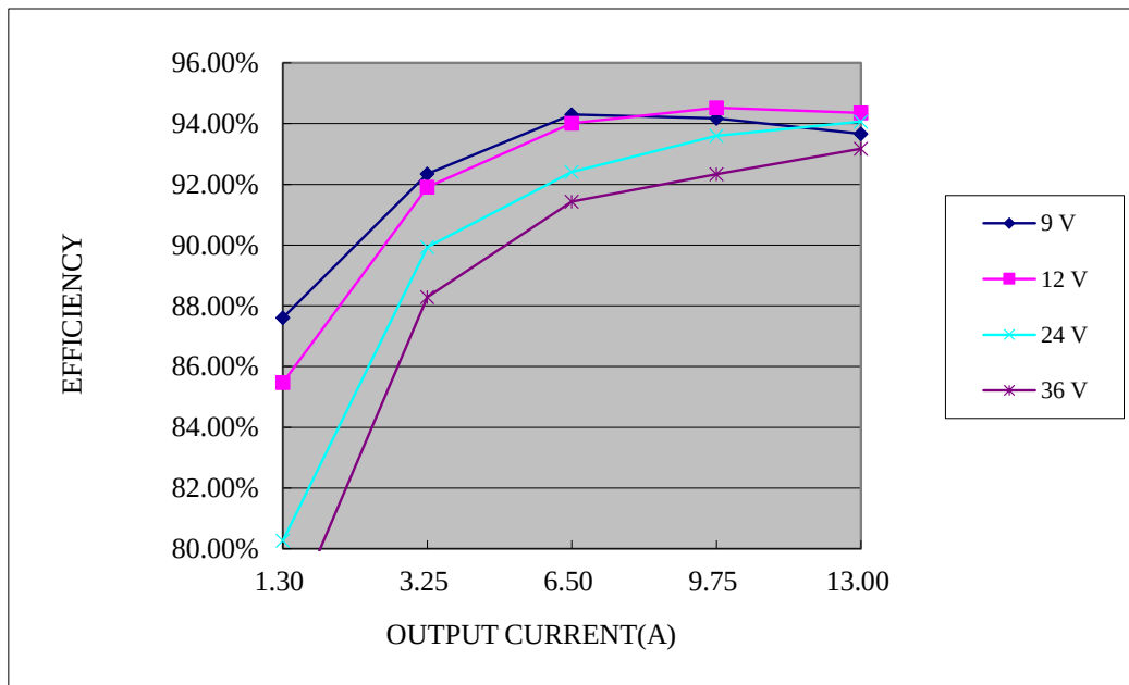
Figure 1. Efficiency data
