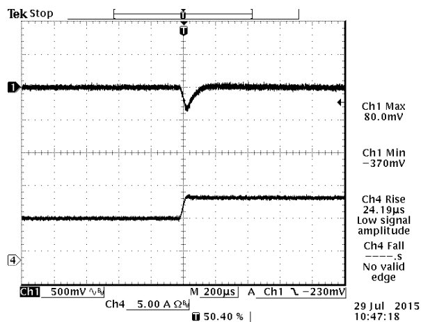
Figure 17. V_{out} = 12\text{ V} 50%-75% Load Transients at V_{in} = 24\text{ V} @ T_a = 25^\circ\text{C}
