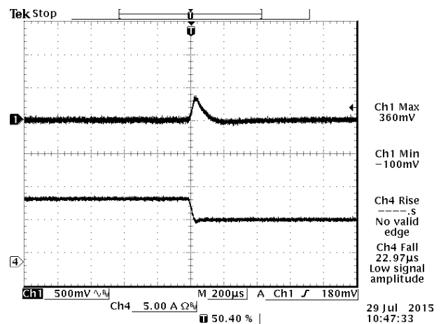
Figure 18. V_{out} = 12\text{ V} 75%-50% Load Transients at V_{in} = 24\text{ V} @ T_a = 25^\circ\text{C}
