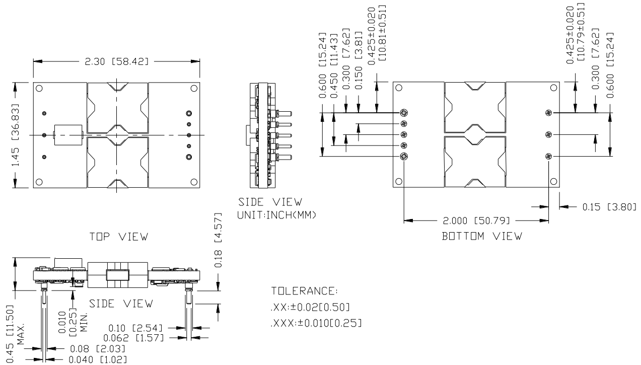
Figure 38. 0RQB-C2Q12V Outline
