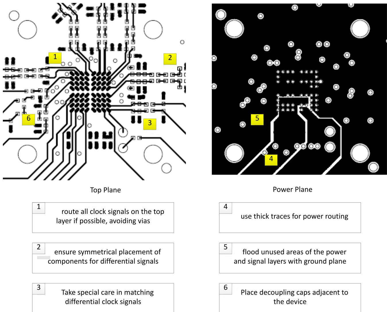
Figure 28. Layout Example, BGA Package
