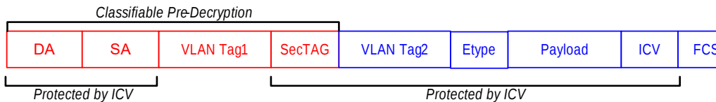
Figure 31 • MACsec Transform to Single and Dual Tag Bypass
