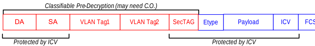
Figure 32 • EoMPLS with One Label
