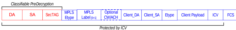
Figure 33 • Standard and Advanced MACsec Transform
