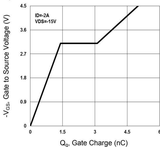
Figure 4. Gate Charge Waveform
