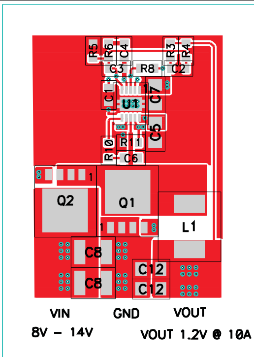
Figure 16. Top Copper With Components
