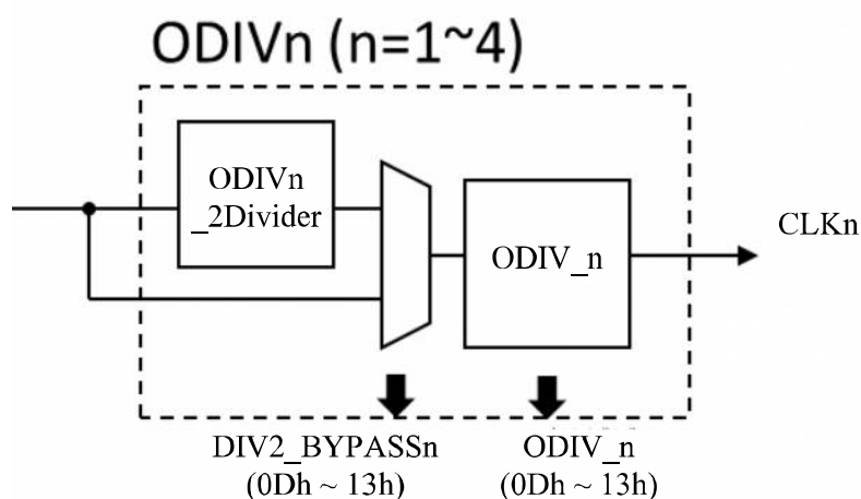
Figure 14. ODIVn configuration
