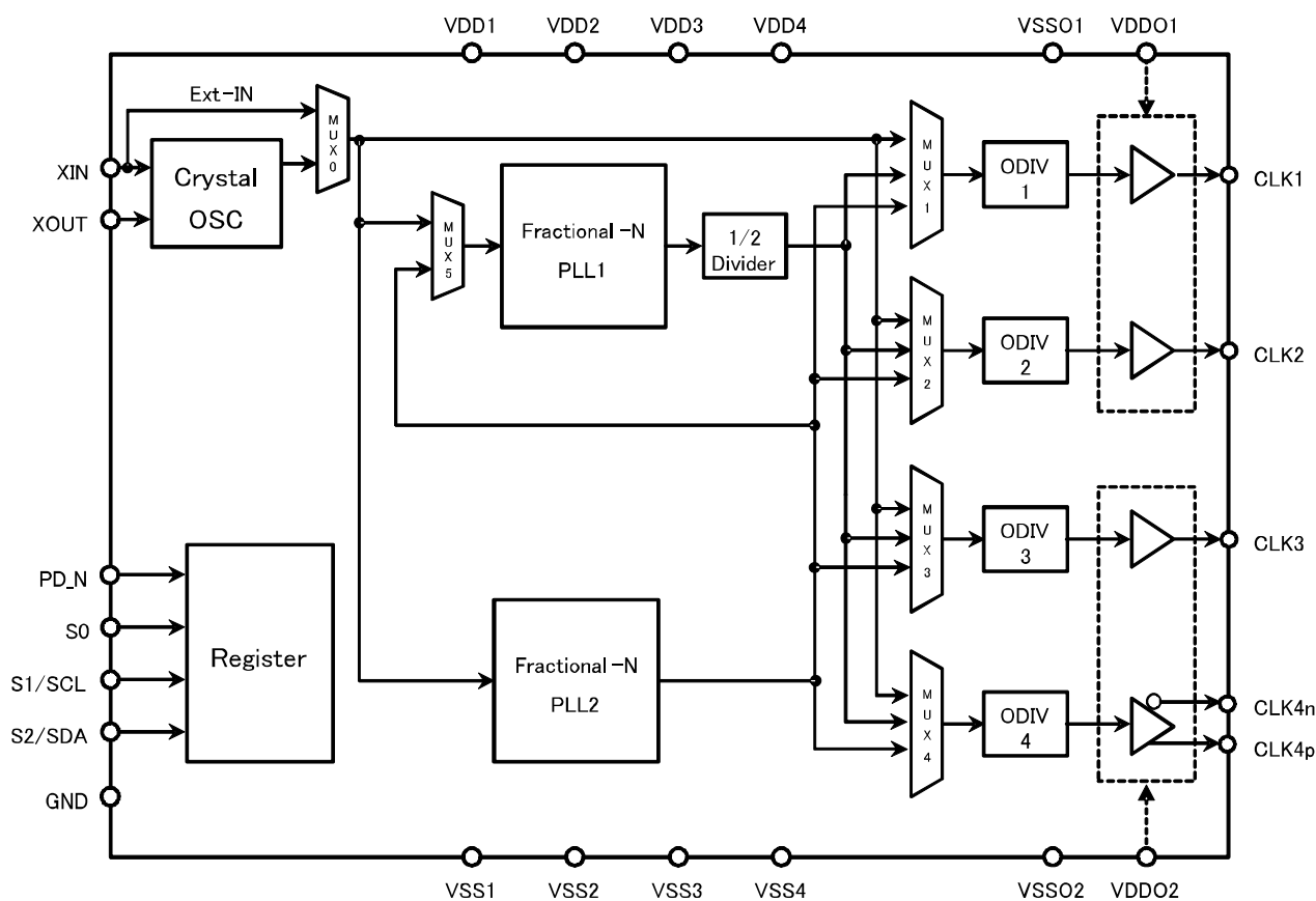
Figure 1. AK8140A Programmable Multi Clock Generator with XO
