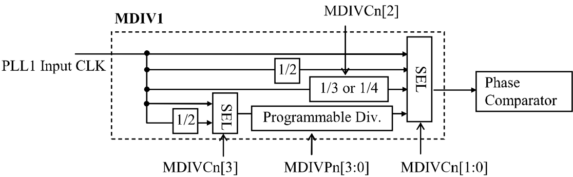
Figure 16. MDIV1 Configuration
