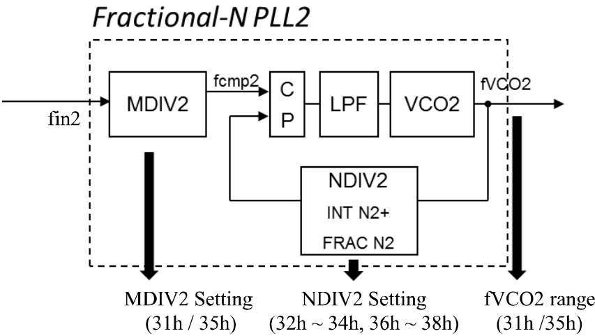
Figure 17. PLL2 Block Diagram
