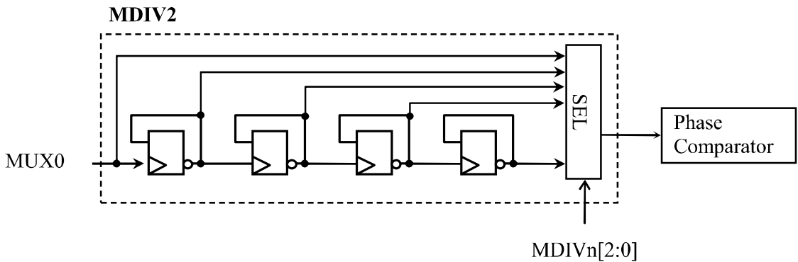
Figure 18. MDIV2 configuration
