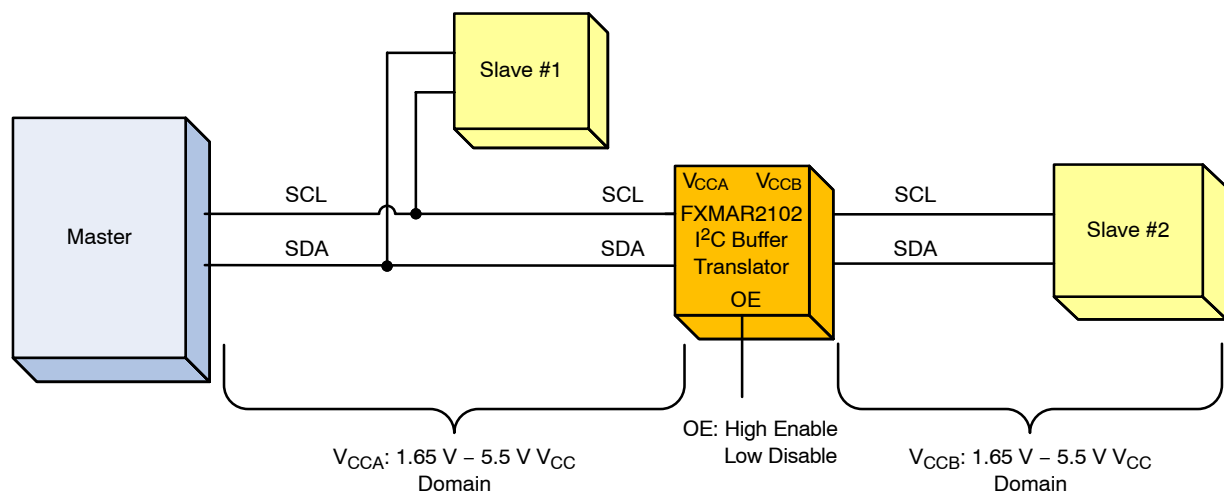
Figure 7. Bus Isolation
