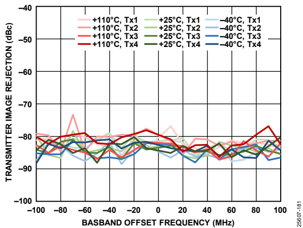
Figure 252. Transmitter Image Rejection Across Large Signal Bandwidth vs. Baseband Offset Frequency
