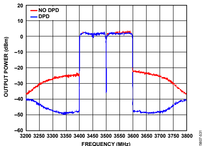
Figure 602. Transmitter Output Spectrum for Normal Operation (Red) and with DPD Activated (Blue) for a 2×, 100 MHz, 5G NR200 Waveform, 37 dBm, LO = 3500 MHz, and R_{BW} = 100 kHz
