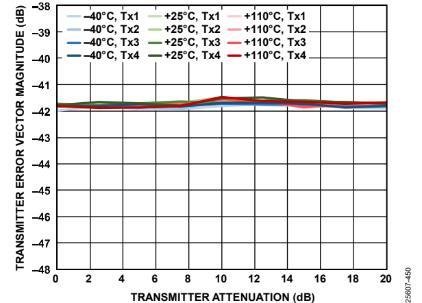
Figure 521. Transmitter Error Vector Magnitude vs. Transmitter Attenuation, 20 MHz LTE Signal Centered at LO Frequency, Sample Rate = 491.52 MSPS, Loop Filter Bandwidth = 400 kHz, Loop Filter Phase Margin = 60°
