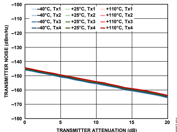
Figure 6. Transmitter Noise vs. Transmitter Attenuation, 10 MHz Offset
