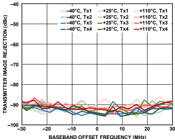
Figure 5. Transmitter Image Rejection Across Large Signal Bandwidth vs. Baseband Offset Frequency
