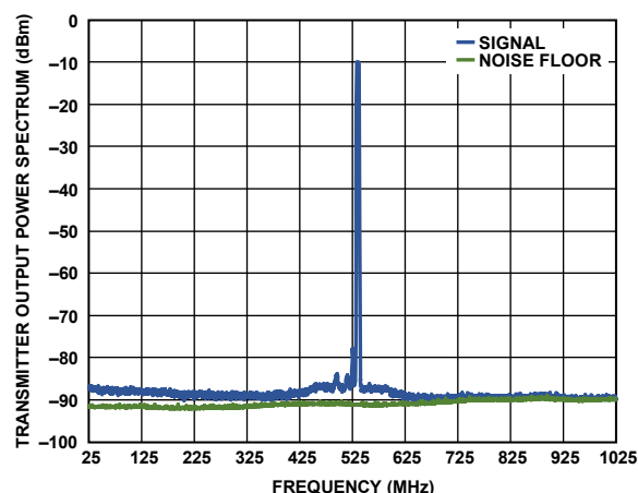
Figure 4. Transmitter Output Power Spectrum, Tx1, 5 MHz LTE, 10 MHz Offset, -10 dBFS RMS, 1 MHz Resolution Bandwidth, T j = 25°C
