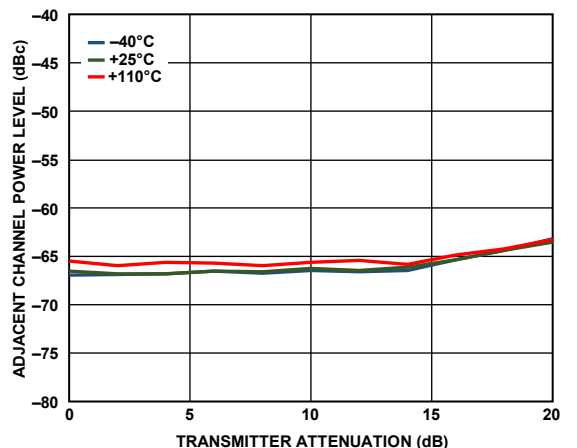
Figure 8. Adjacent Channel Power Level vs. Transmitter Attenuation, 21 MHz Baseband Offset, 5 MHz LTE, Peak to Average Ratio (PAR) = 12 dB
