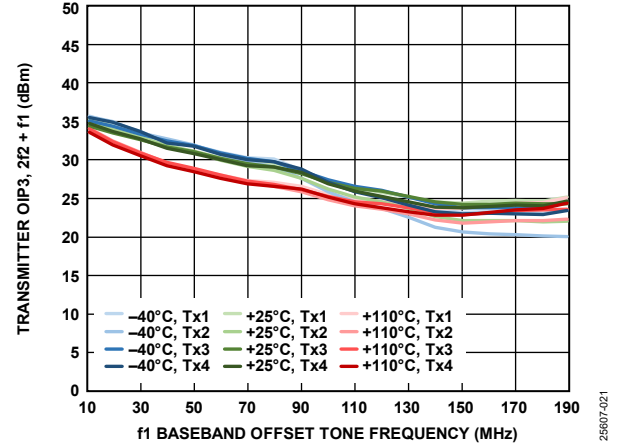
Figure 92. Transmitter OIP3, 2f_2 + f_1 vs. f_1 Baseband Offset Tone Frequency, f_2 = f_1 + 5 MHz, 15 dB Digital Back Off per Tone
