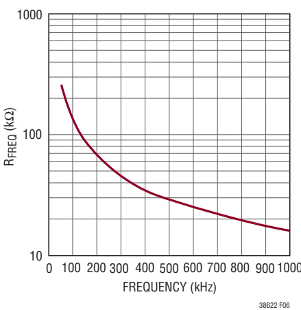
Figure 6. FREQ Pin Resistor Value vs Frequency
